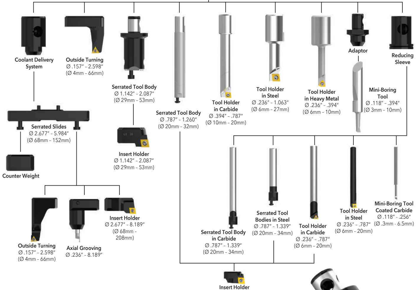
PrimeBore Head
