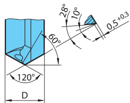
Point grind G for machining cast iron
