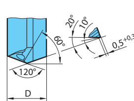
Point grind A for machining aluminium
